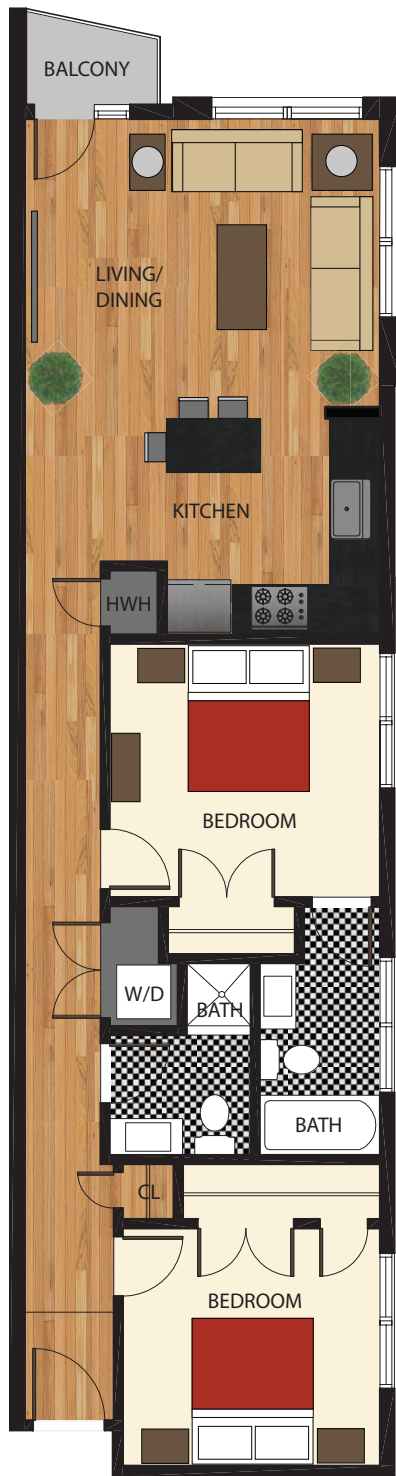
TYPICAL UNIT PLAN SCALE: 1/8"=1'-0"
